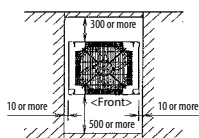
For single unit installation <Pattern 1>
