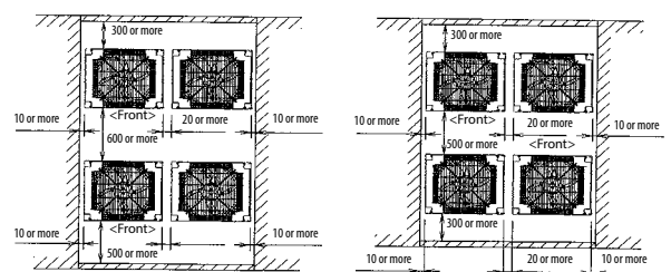
For centralized group layout <Pattern 1>
